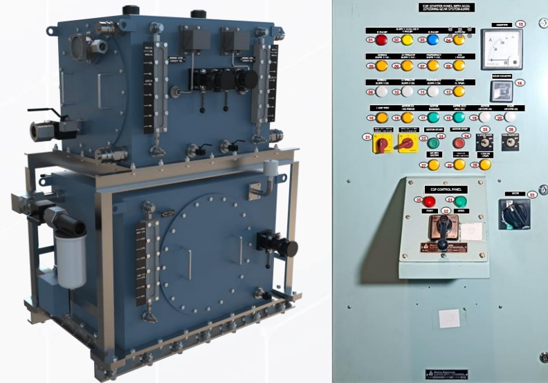
HYDRO-MECHANICAL CONTROLS SYSTEM
